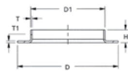
Pressed collars
